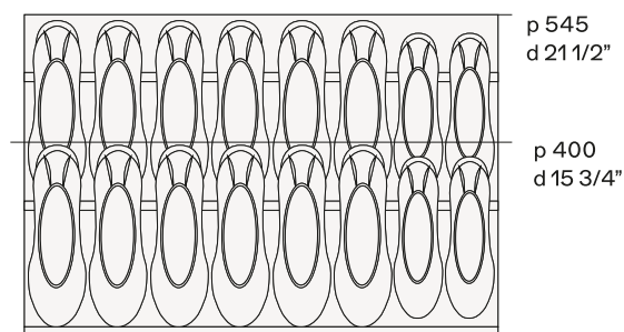
Width 30 3/4"
