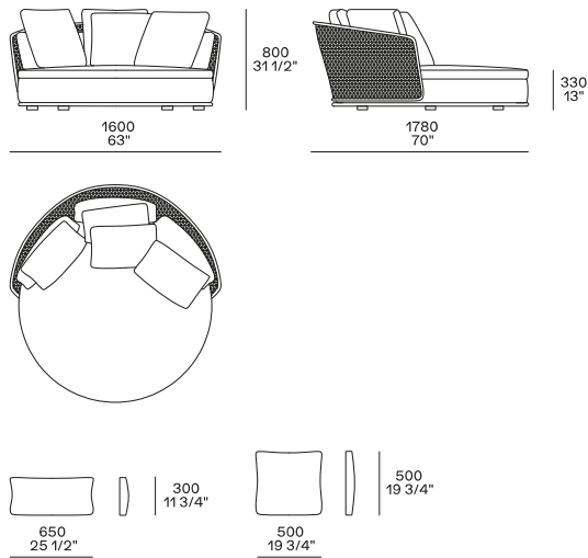
Backrest and backrest cushion
